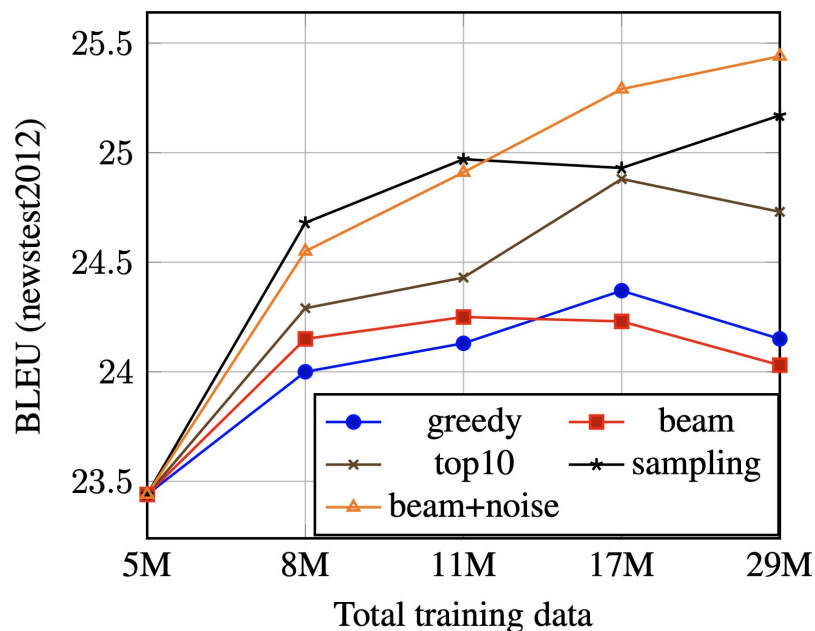
High-resource: diversity matters
