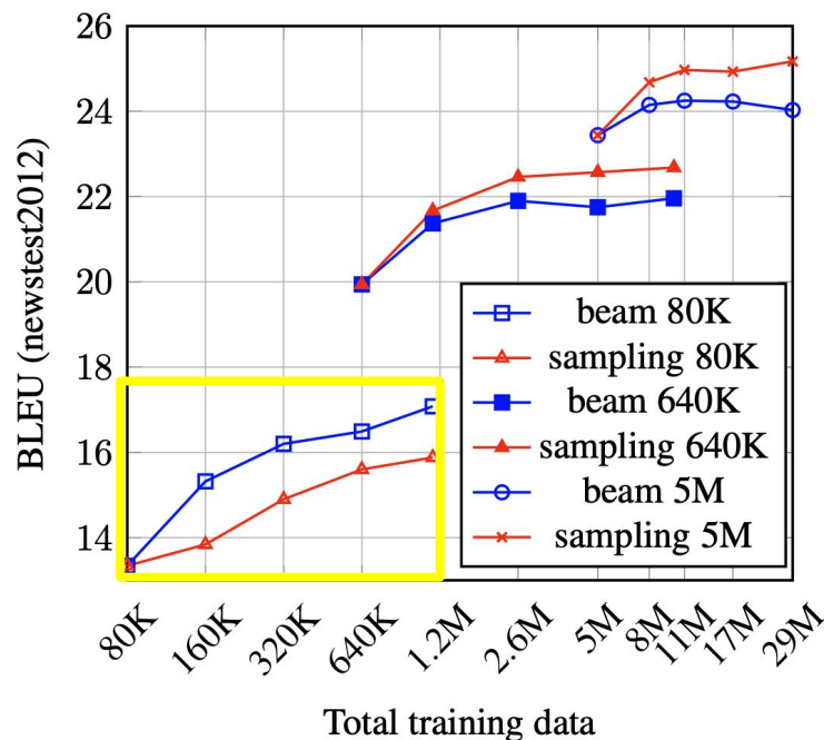
Low-resource: quality matters
