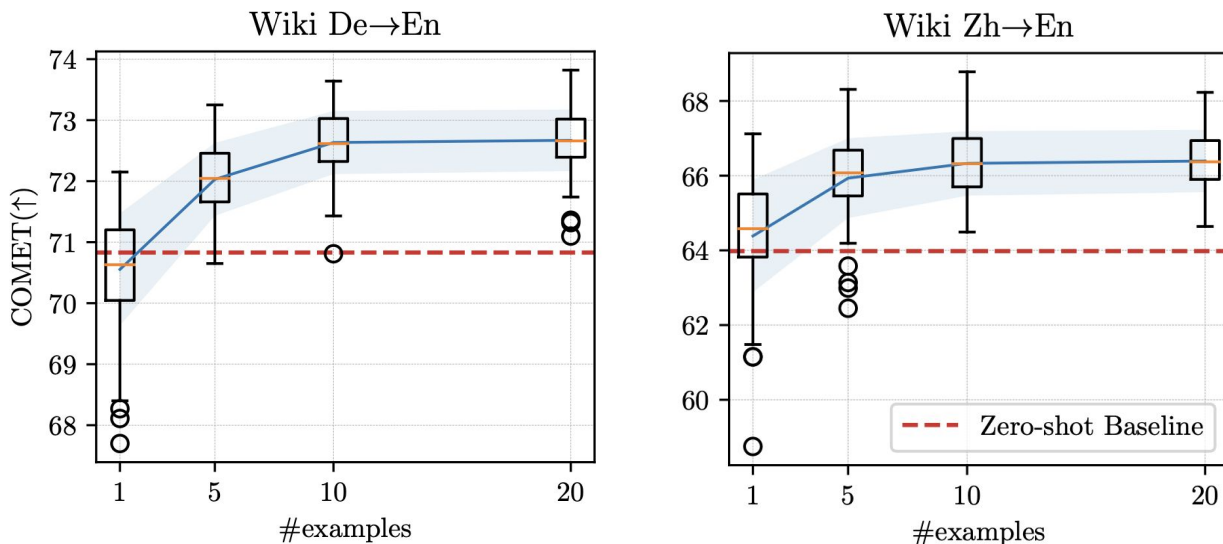
Figure 1: COMET scores for few-shot prompting as a function of the number of prompt examples ( K = 1, 5, 10, 20 ) on Wiki Ablation sets. For each setup, we randomly sample 100 times from the example pool and show the performance distribution via box plots. Dashed red line denotes the zero-shot baseline; blue curve and shadow area denote the mean and standard deviation.
